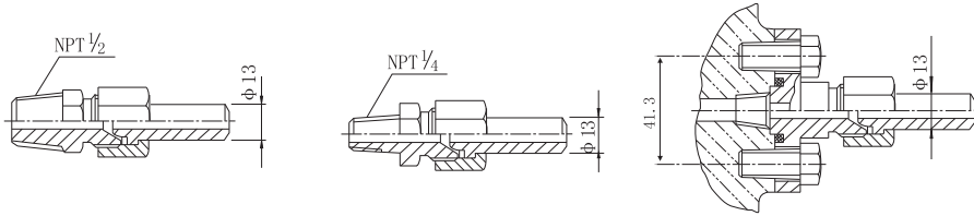
NPT 1/2外螺纹接头
